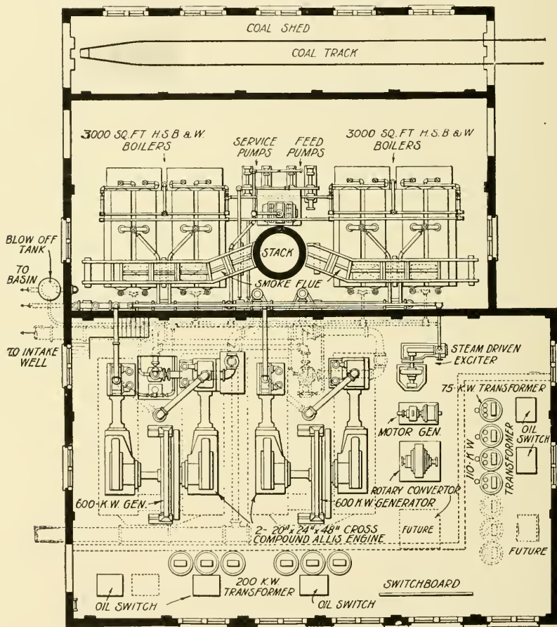
Fig. 146. Plan of Winona Railway Company Power House
